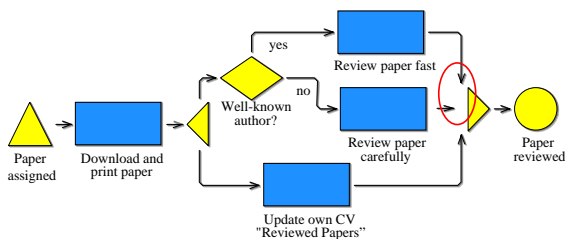
Figure 5: Invisible Merge in ADONIS ®
