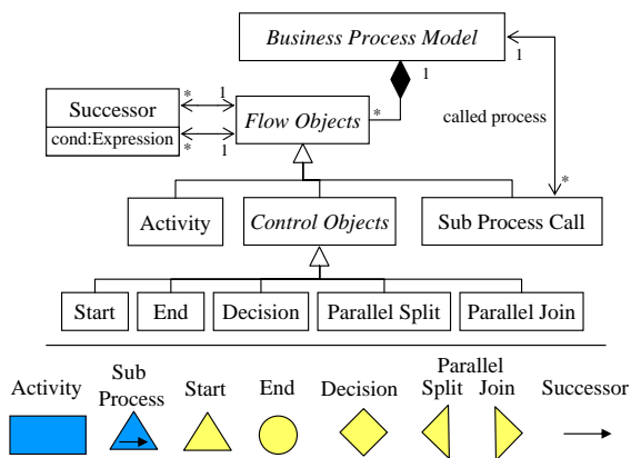
Figure 1: Part of the ADONIS ® BP meta model and the concrete syntax
